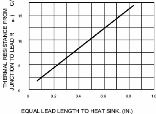
FIG.5-TYPICAL THERMAL RESISTANCE
