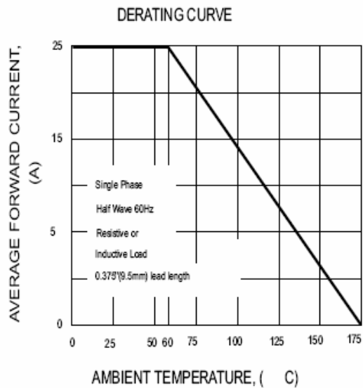
FIG.1-TYPICAL FORWARD CURRENT
