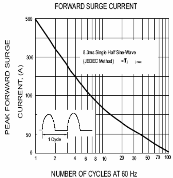
FIG.2-MAXIMUM NON-REPETITIVE PEAK
