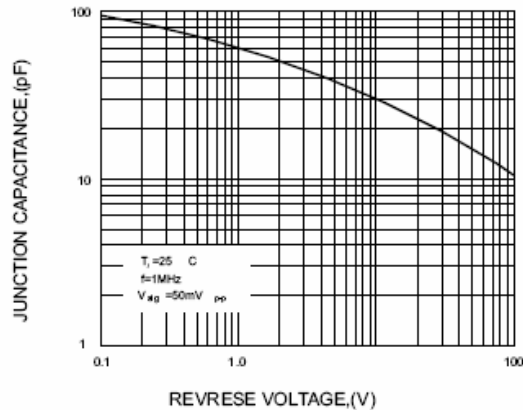
FIG.5-TYPICAL JUNCTION CAPACITANCE
