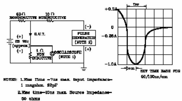
FIG.5-TEST CIRCUIT DIAGRAM AND REVERSE RECOVERY TIME CHARACTERISTIC
