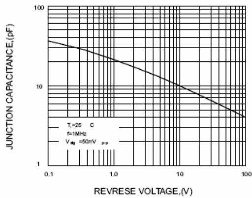
FIG.5-TYPICAL JUNCTION CAPACITANCE
